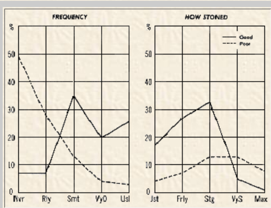
Figure 20-2. QUALITY OF NIGHT'S SLEEP AFTER GOING TO BED STONED Note.—For guide to interpreting the "How Stoned" graph, see note on Figure 6-1.
